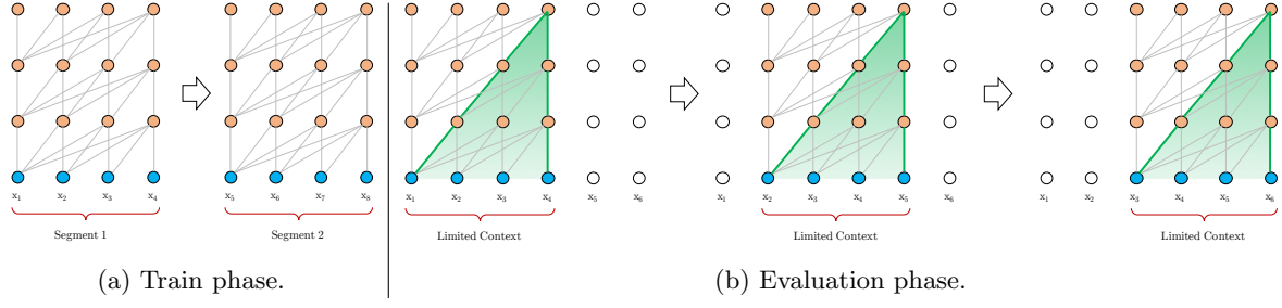
Figure 32: Illustration of the vanilla transformer model with a segment length 4. [DYY + 19]
