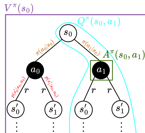
Figure 2: Backup diagram illustrating the different value functions.
